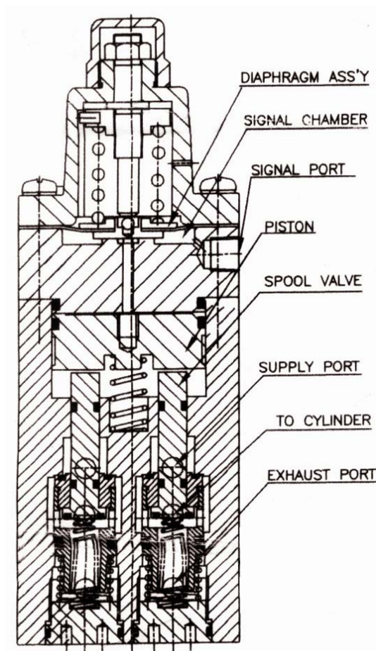
Change Over Valve (DCV02) Double acting
