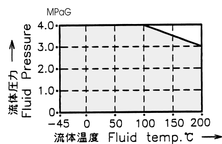
Fig. 3-1 TEFLON SHEET
