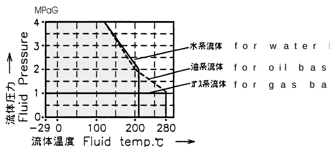
Fig. 3-2 JOINT SHEET
