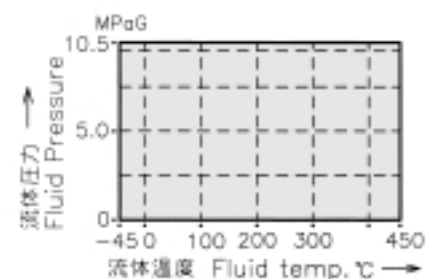
Fig. 3-3 GRAFOIL SHEET
